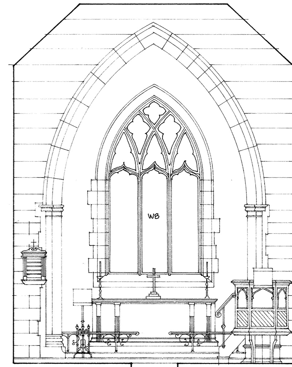
SECTION 'BB' FROM DRAWING NO C
