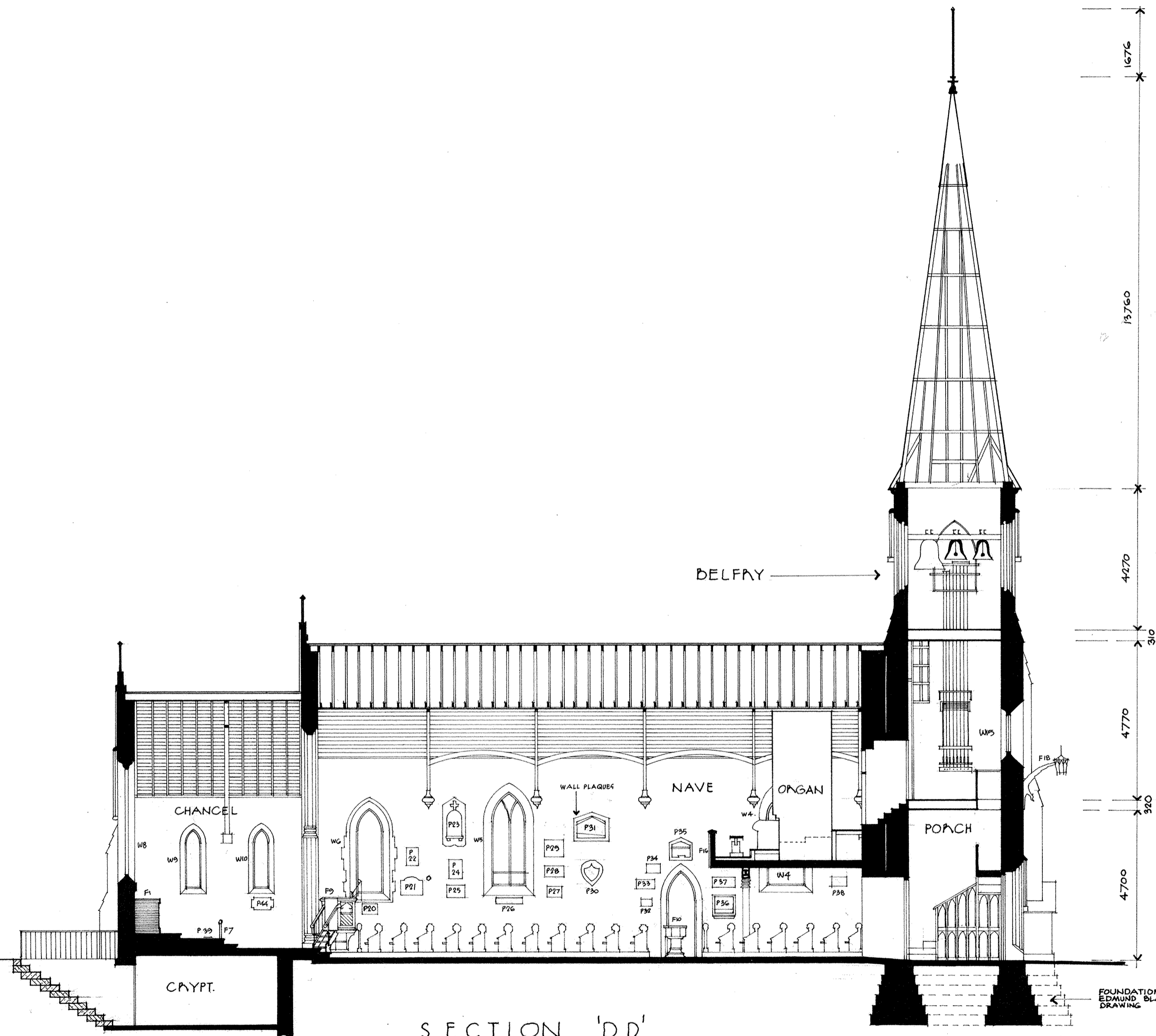
ANGLICAN CHURCH OF ST. JOHN THE BAPTIST, CANBERRA. MEASURED DRAWING.
