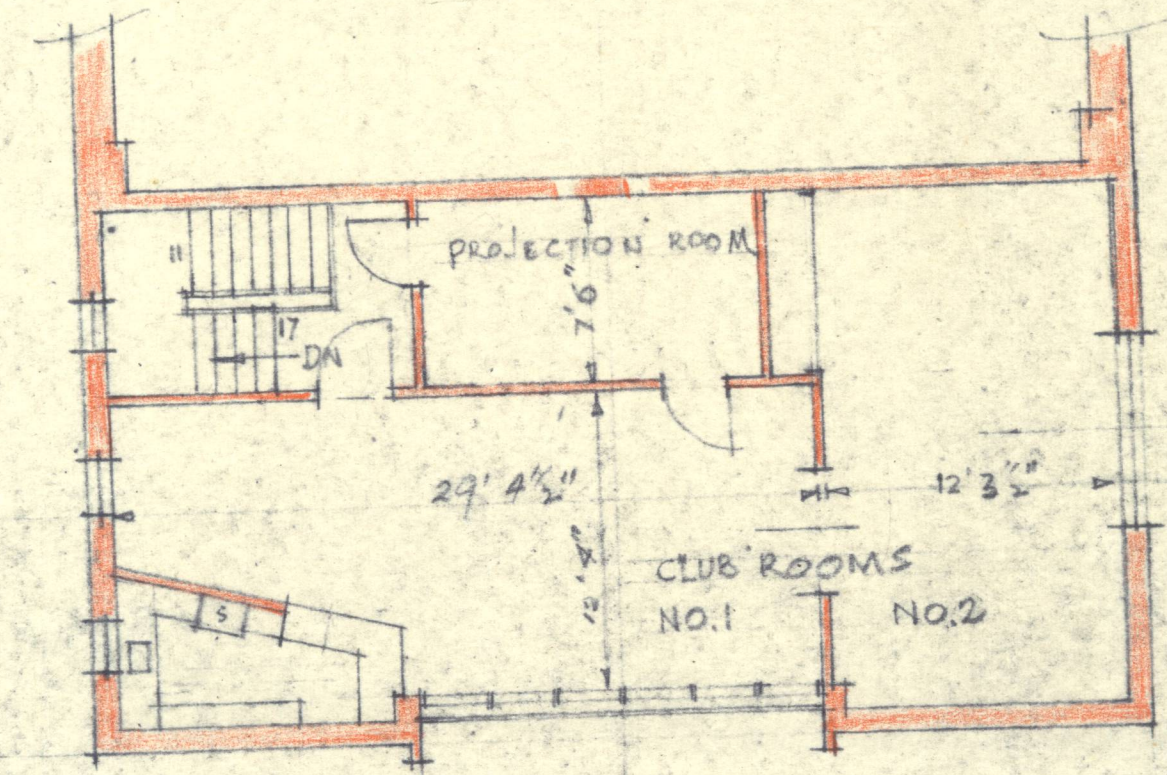
FIRST FLOOR PLAN (OVER FOYER & TOILETS)
